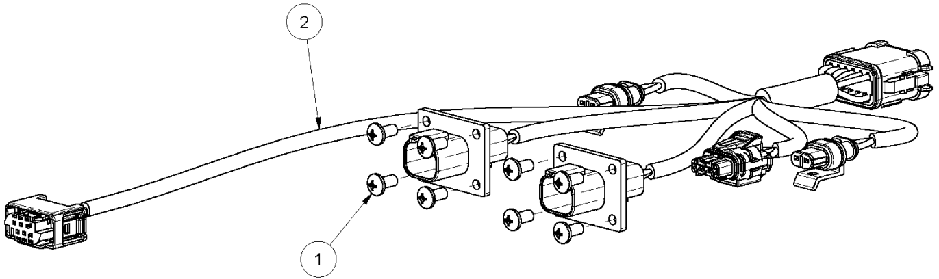
4CM00054 - SERVICE KIT - WIRING HARNESS AND FASTENERS, CONTROL MODULE
